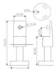
Adjustable Support Leg Width Selection is available (Optimum width: 12-18mm) Height Selection is available (Optimum height: 90-115mm)
