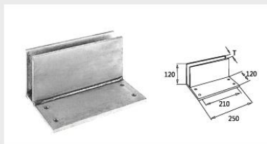
JRS-8633 玻璃托架 Glass bracket
