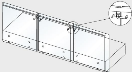
JRS-8633 玻璃托架 Glass bracket
