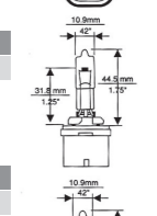
PGJ13 IEC 7004-107
