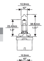
PG13 IEC 7004-107
