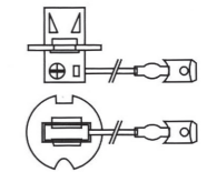
PK22s IEC 7004-47
