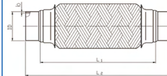
With nipple (extension tube)
