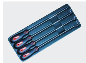
Handle: hard pp core, soft TPE cover with round cross-section, Blade: round, satin chrome plated, Cr-V steel, hardness 52HRc
