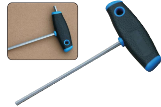
Handle: 2-component, T-shaped hard PP cover, soft TPR cover. Blade: round, two-sided, black finish, surface point tips.
