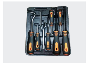
Handle: hard pp core, soft TPE cover with round cross-section, Blade: round, chrome plated, carbon steel
